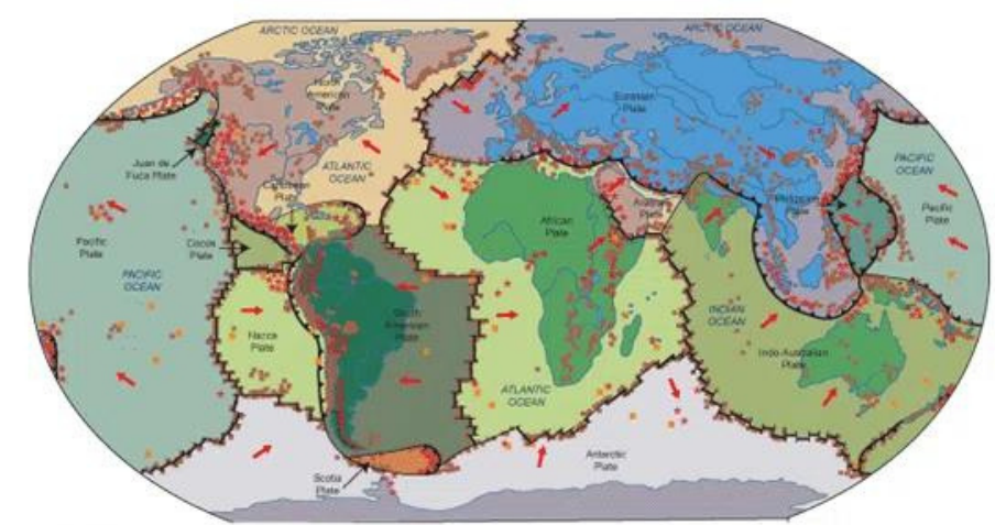
FIGURE 1 The distribution of active earthquakes and volcanoes shows us where the earth's plates are crashing together or pulling apart. Here we find "explosive volcanoes." In the middle of some plates are hot spots, like the Hawaiian islands, where hot rocks from the interior feed a different kind of volcano called "shield volcanoes."
