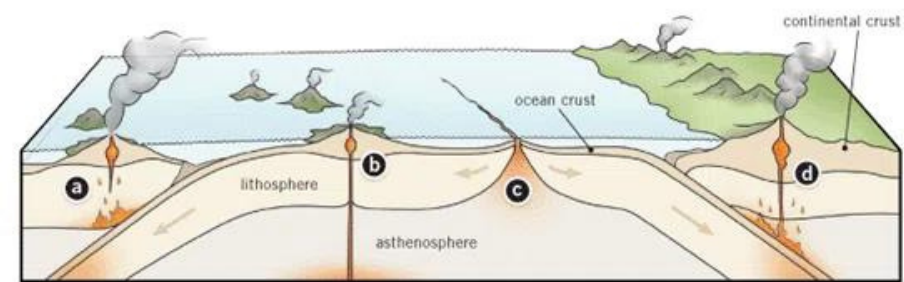
FIGURE 2 (a-d) This diagram depicts three types of volcanoes: (a,d) explosive volcanoes formed where one plate is sinking under another, (b) shield volcanoes formed by plumes of hot rock rising from the earth's interior, and (c) volcanic ridges formed where two plates are pulling apart.
